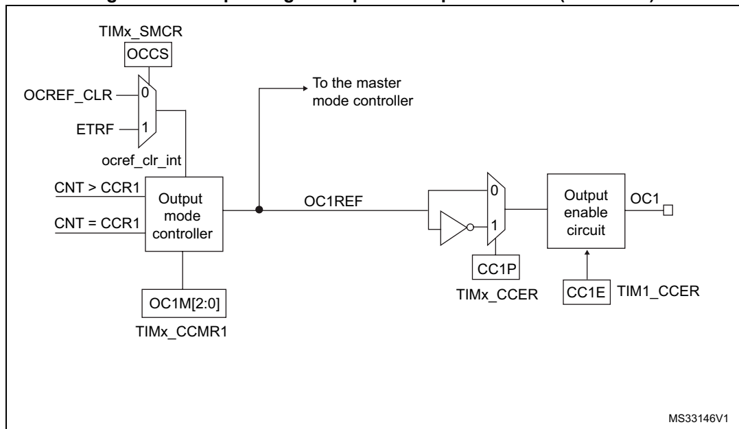
Figure 138. Output stage of capture/compare channel (channel 1)
