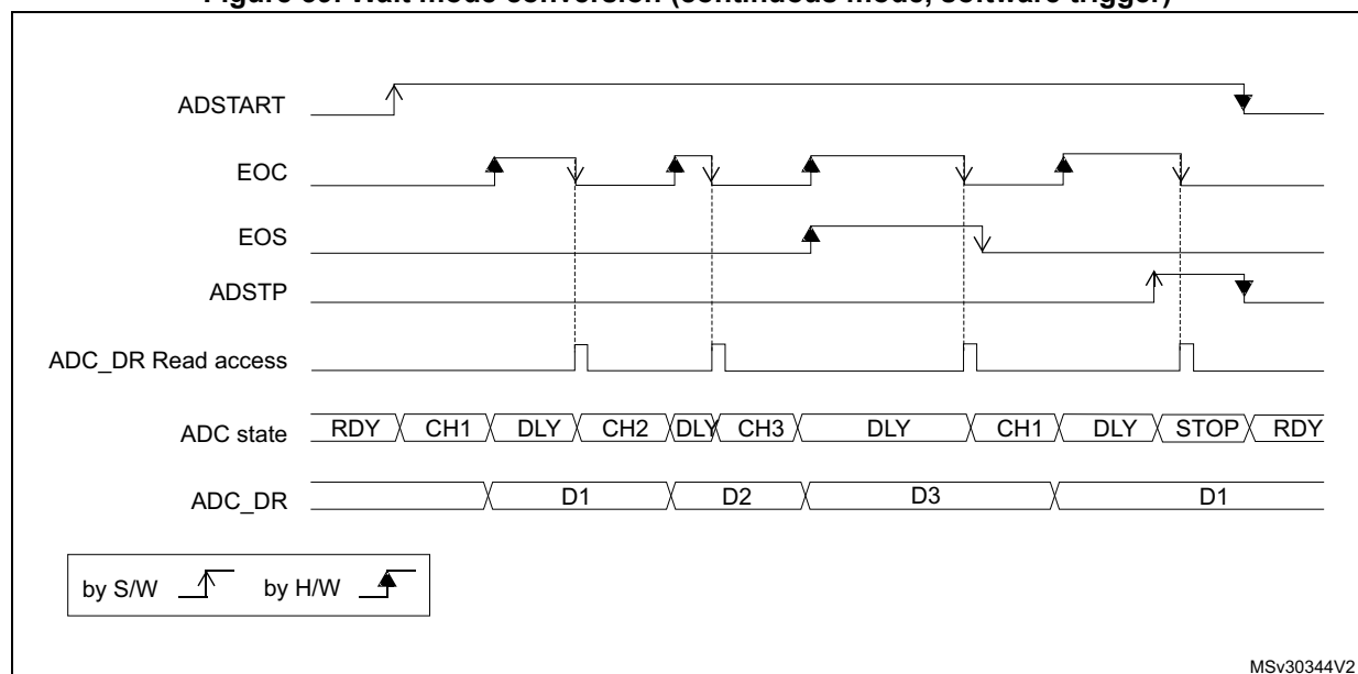
Figure 39. Wait mode conversion (continuous mode, software trigger)
